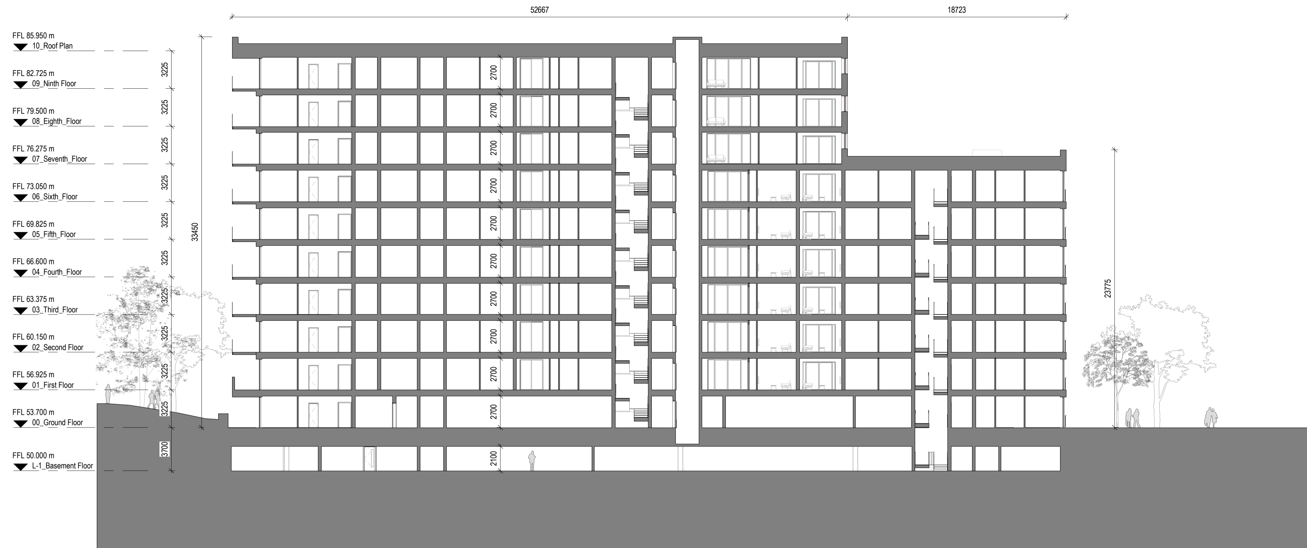
A Block 1D_Cross Section A 1 : 200
