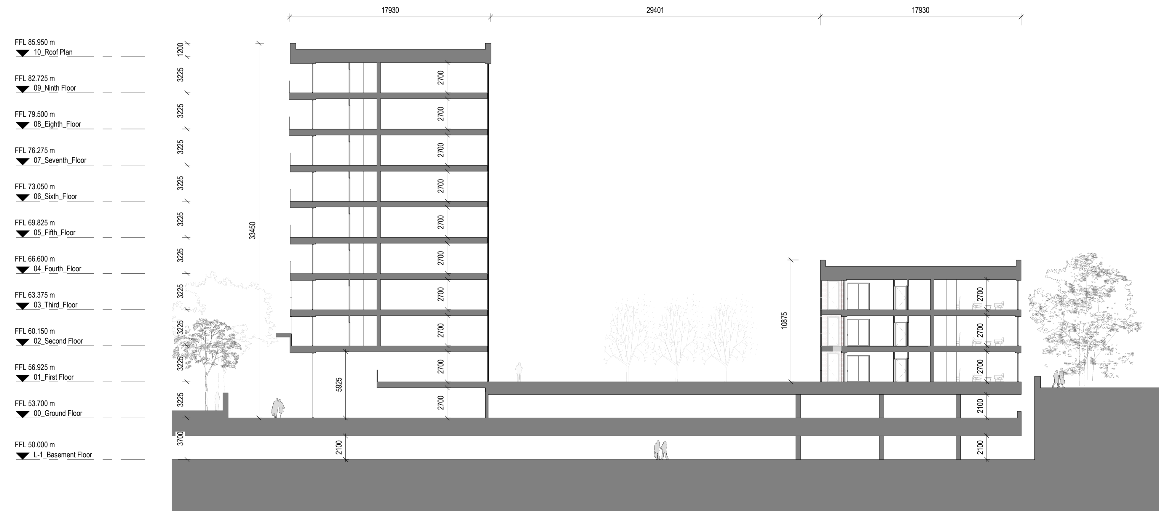
B Block 1D_Cross Section B 1 : 200
